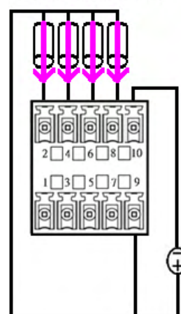
Digital Output Wiring
